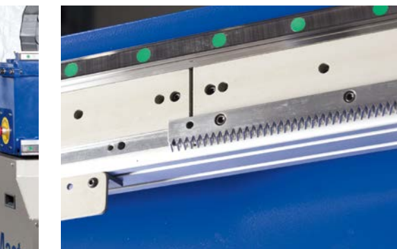
Helical drive gears with linear guides give precision and a smooth drive for top quality cuts and accuracy
